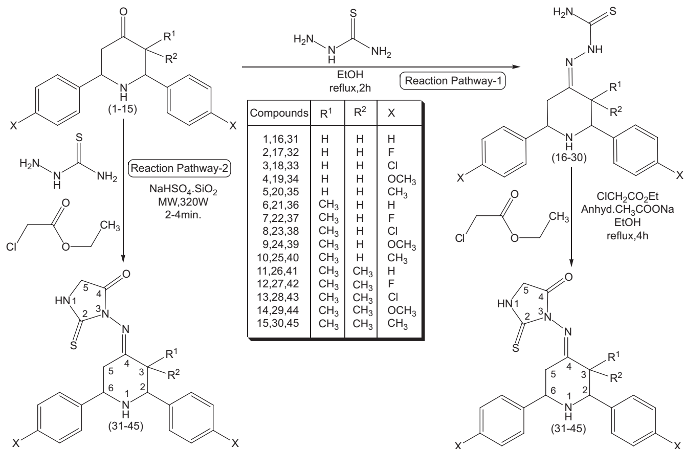
Scheme 1. A facile synthetic route for the synthesis of 3-(3-substituted-2,6-diarylpiperidin-4-ylideneamino)-2-thioximidazolidin-4-ones.
